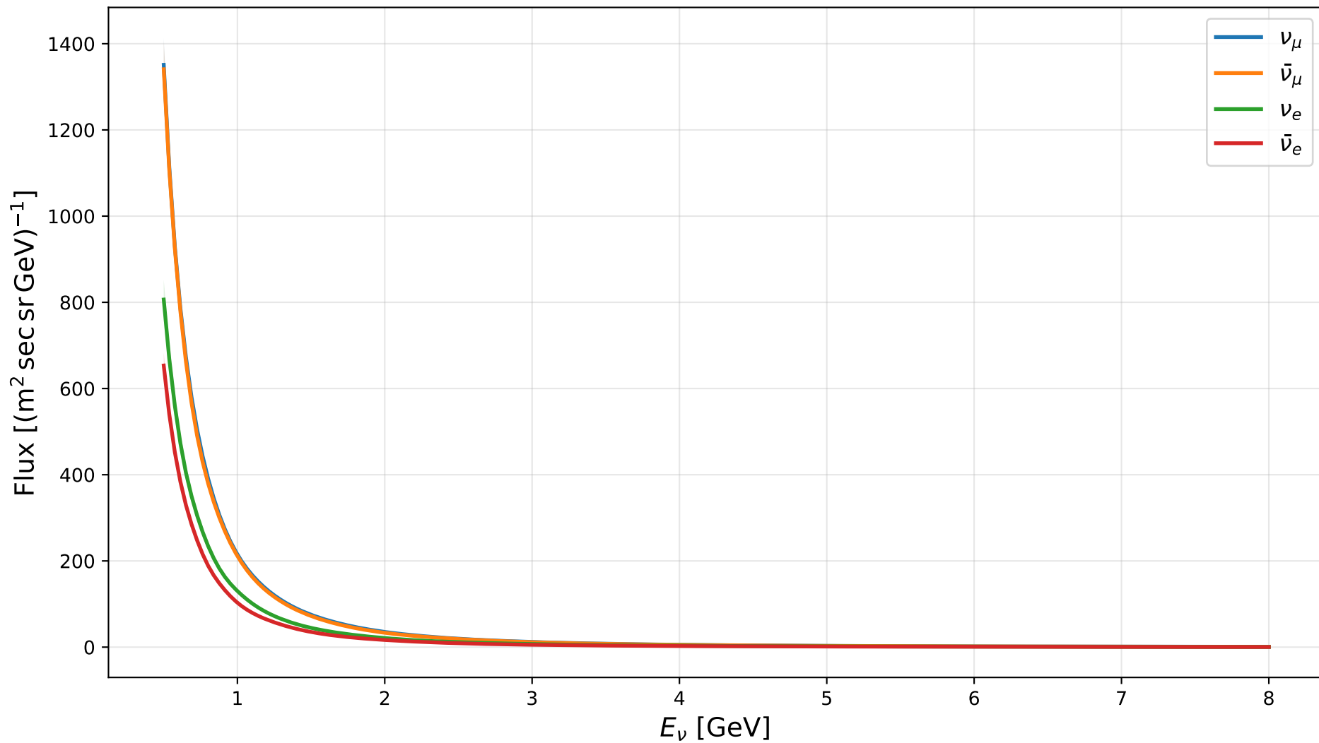
Atmospheric neutrino fluxes at \cos \theta = 0.00
