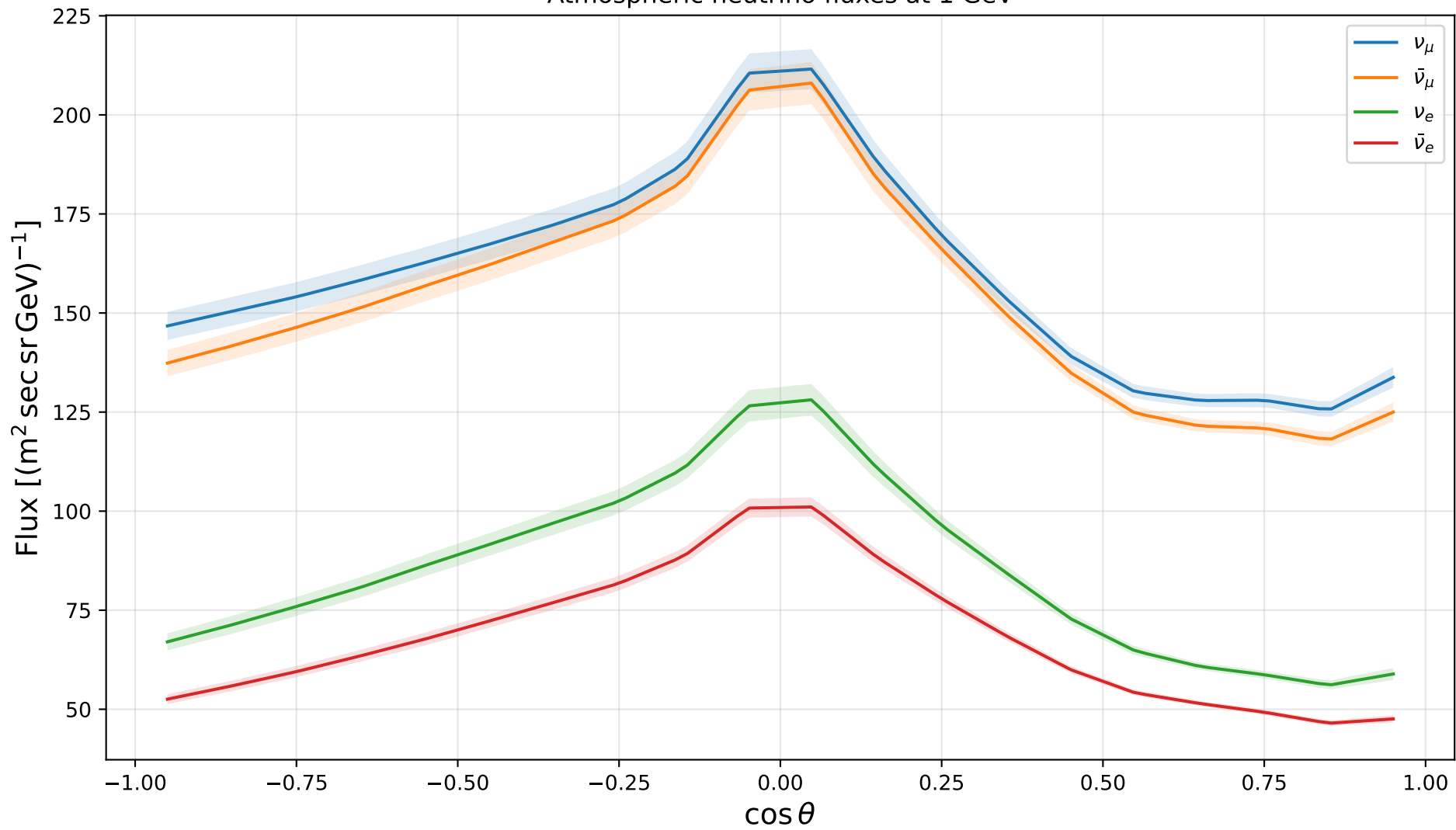
Atmospheric neutrino fluxes at 1 GeV
