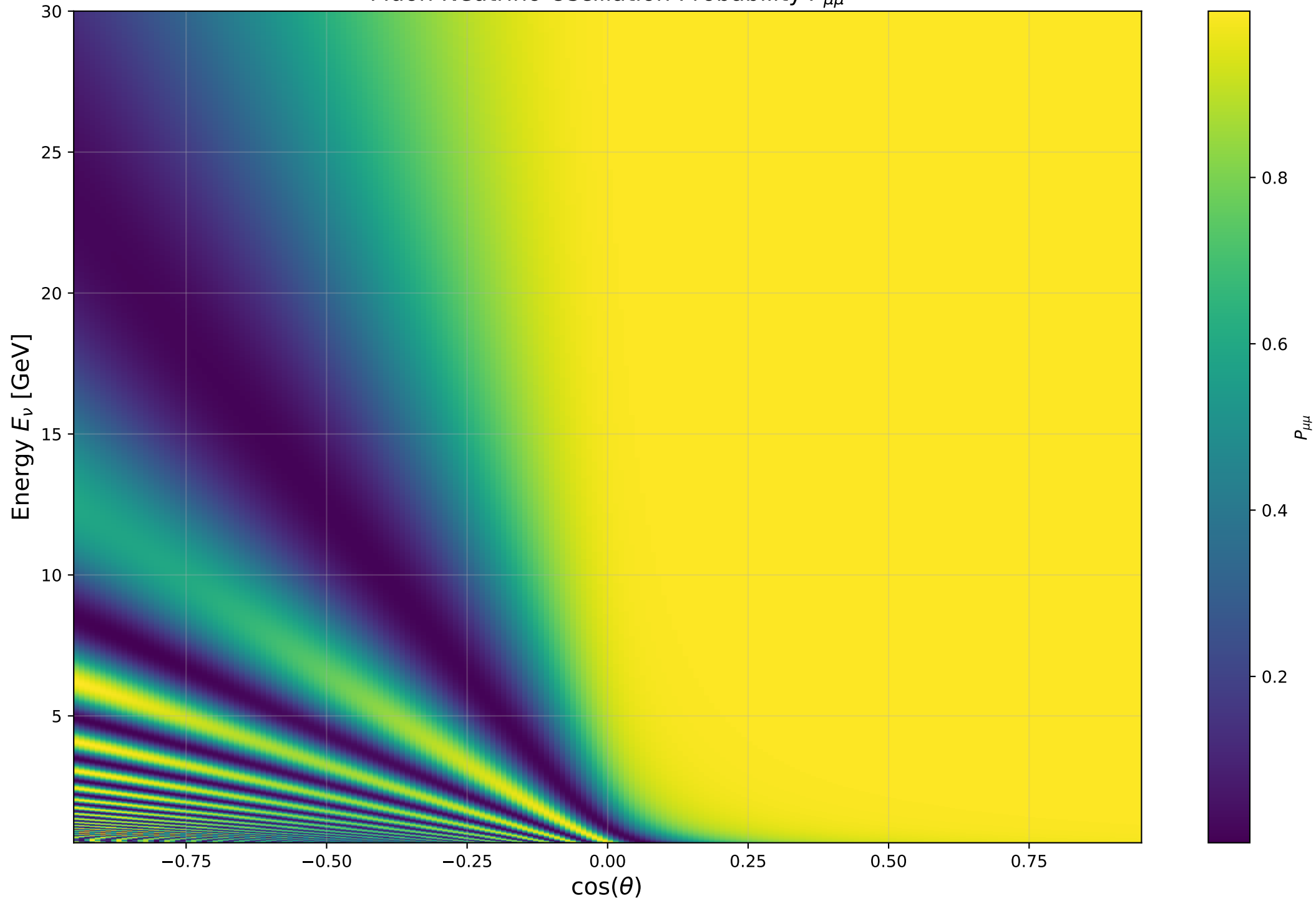
Muon Neutrino Oscillation Probability P_{\mu\mu}
