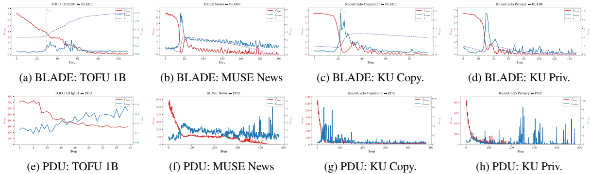
Figure 5: Training dynamics across benchmarks (MUSE Books in main paper, Figure 4). Top: BLADE shows consistent three-phase convergence. Bottom: PDU exhibits recurring oscillations.
