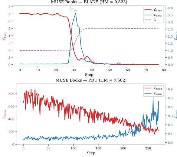
Figure 4: Training dynamics on MUSE Books. Top: BLADE (warm-up → spike-and-ratchet → smooth convergence). Bottom: PDU (recurring oscillations). Full dynamics across all benchmarks in Appendix E.
