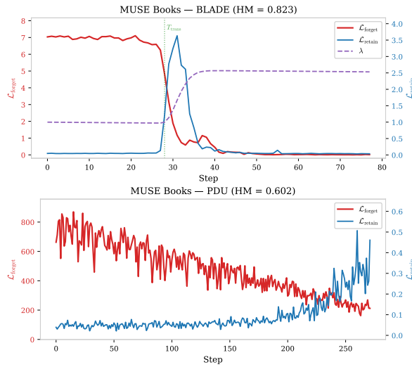
Figure 4: Training dynamics on MUSE Books. Top: BLADE (warm-up → spike-and-ratchet → smooth convergence). Bottom: PDU (recurring oscillations). Full dynamics across all benchmarks in Appendix ??.
