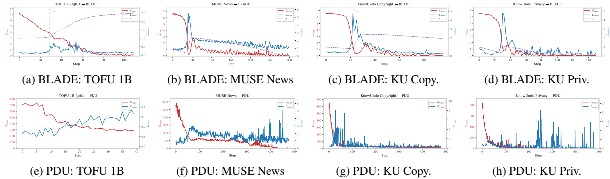
Figure 5: Training dynamics across benchmarks (MUSE Books in main paper, Figure ??). Top: BLADE shows consistent three-phase convergence. Bottom: PDU exhibits recurring oscillations.
