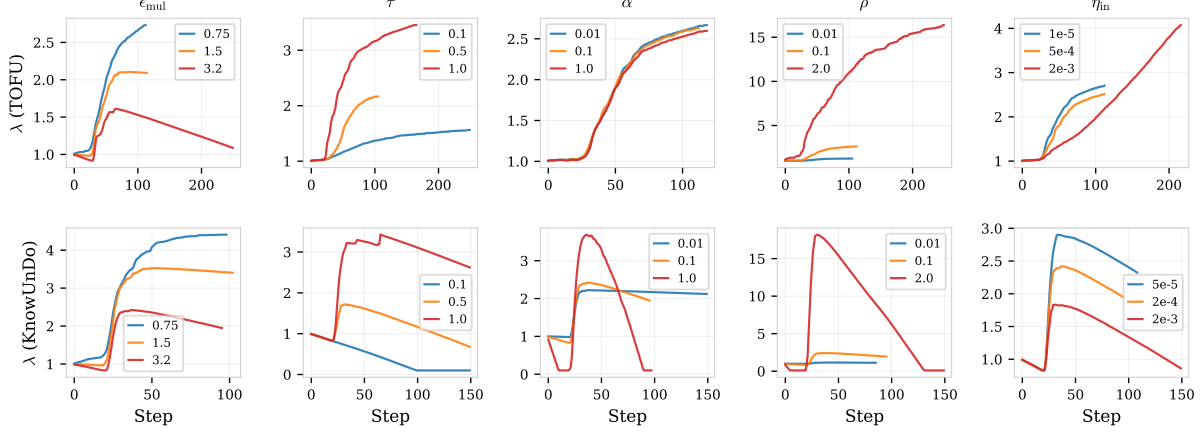
Figure 9: Representative \lambda trajectories under hyperparameter sweeps. Top: TOFU. Bottom: KnowUnDo. Each panel shows three values (low/mid/high) for one parameter. The dual variable adapts its trajectory to compensate for parameter changes, explaining the robustness in Figure 8.
