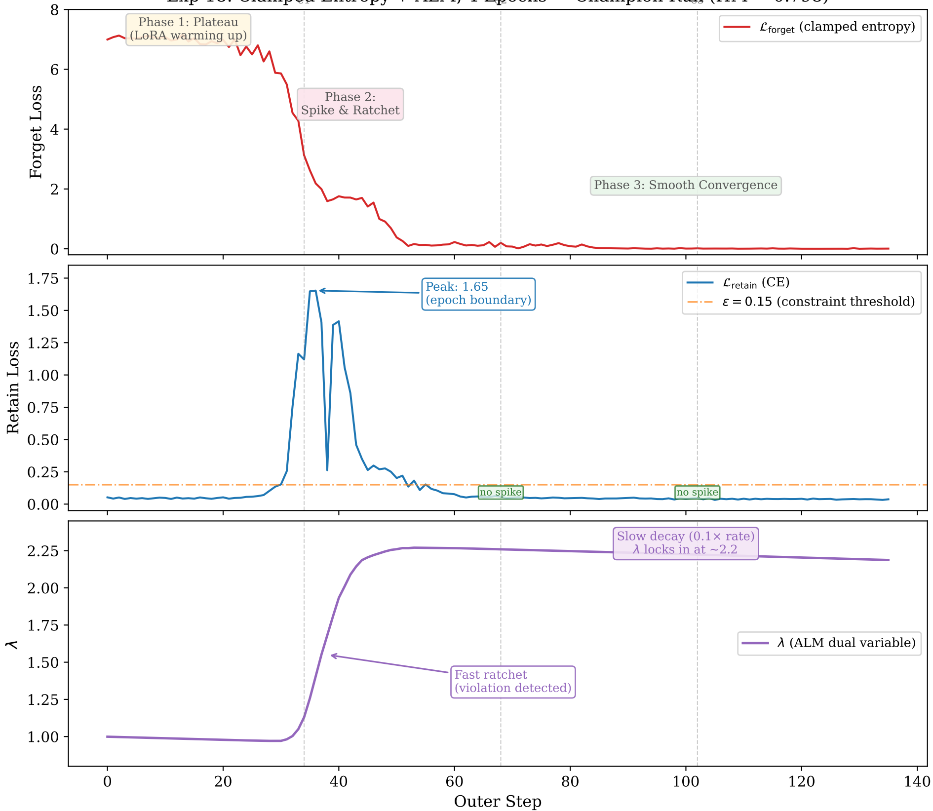
Exp 18: Clamped Entropy + ALM, 4 Epochs — Champion Run (HM = 0.798)
