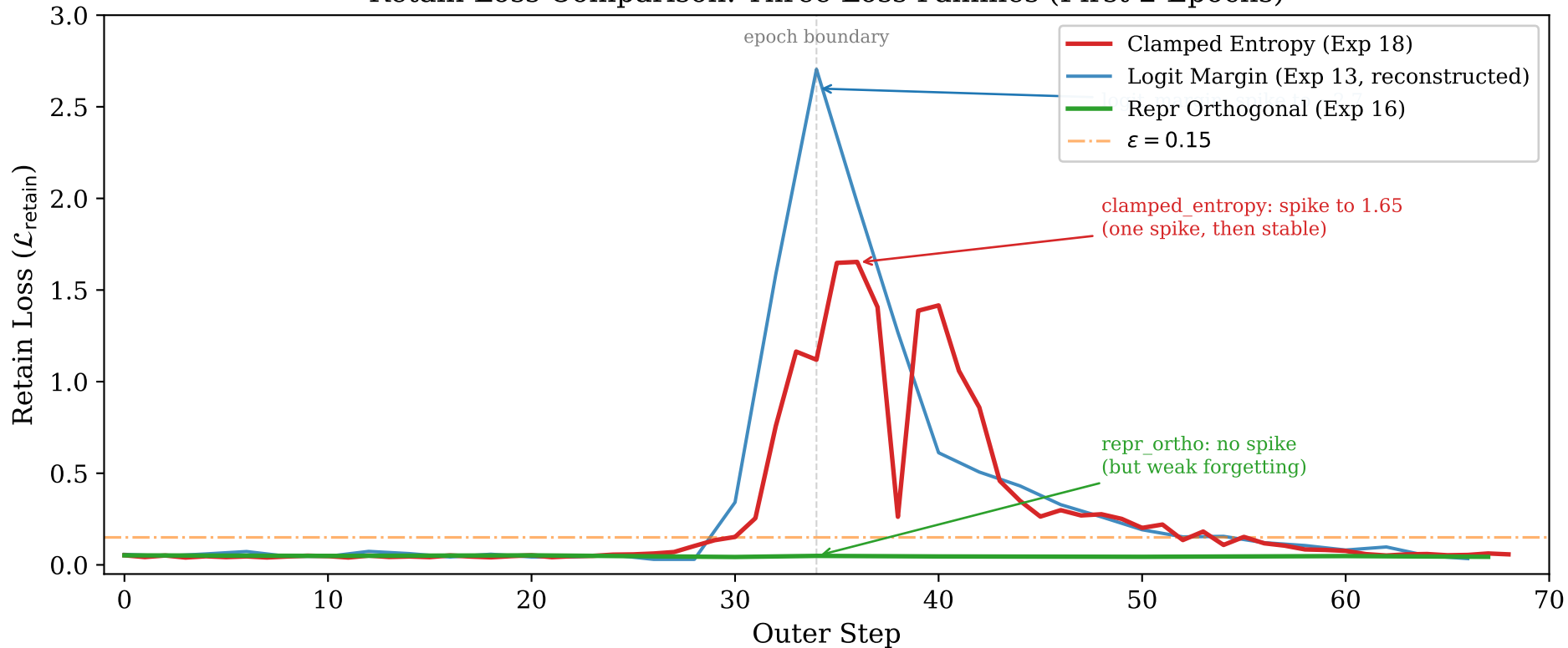
Retain Loss Comparison: Three Loss Families (First 2 Epochs)
