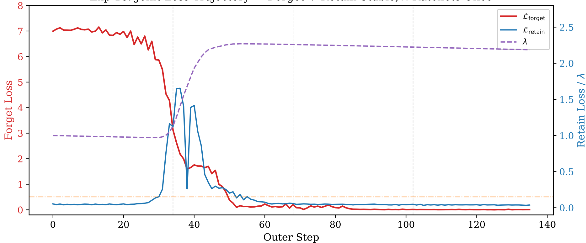
Exp 18: Joint Loss Trajectory — Forget \downarrow Retain Stable, \lambda Ratchets Once
