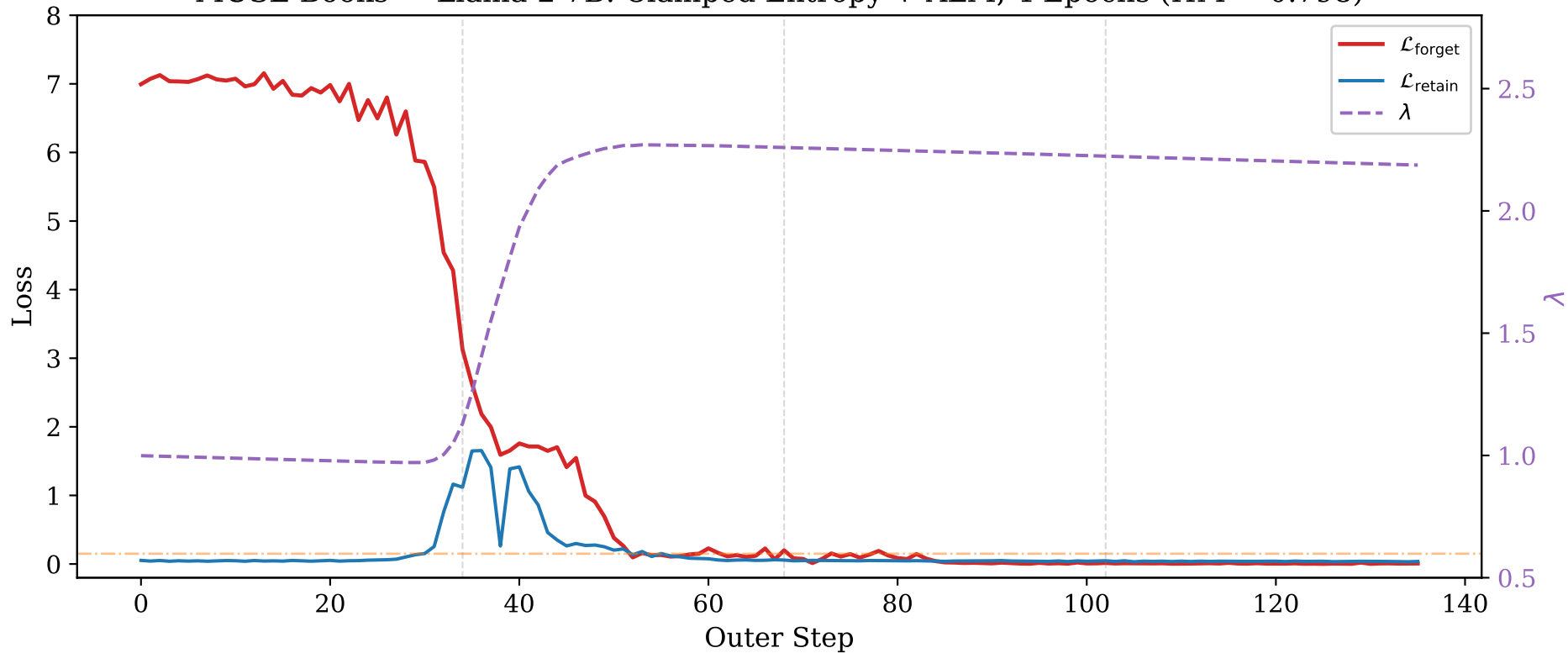
MUSE Books — Llama-2-7B: Clamped Entropy + ALM, 4 Epochs (HM = 0.798)
