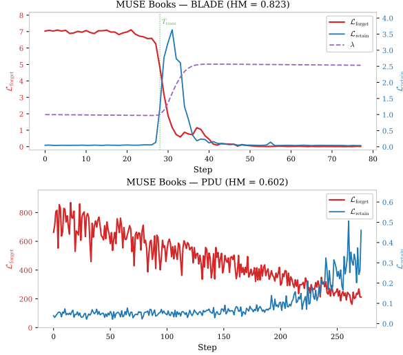
Figure 4: Training dynamics on MUSE Books. Top: BLADE (warm-up → spike-and-ratchet → smooth convergence). Bottom: PDU (recurring oscillations). Full dynamics across all benchmarks in Appendix E.
