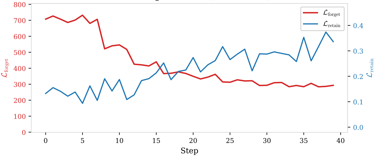
TOFU 1B fgt01 — PDU (HM = 0.690)
