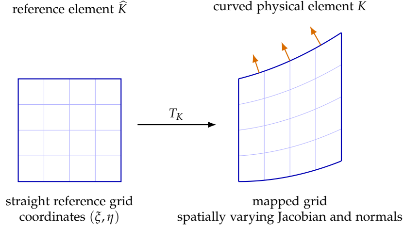
Figure 3.4: An illustrative polynomial map T_K(\tilde{\xi}, \eta) = (\tilde{\xi}, (1 + \tilde{\xi}/4)\eta + \tilde{\xi}^2/5) from the unit square. Its determinant is 1 + \tilde{\xi}/4 > 0 : equal reference areas need not have equal physical areas. Orange arrows show outward normal directions along the curved top face (not their magnitudes). The interior lines are coordinate lines within one element, not separate DG cells. This is a geometric schematic, not a mesh from a numerical experiment.
