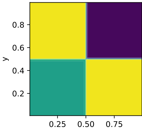
RKDG
