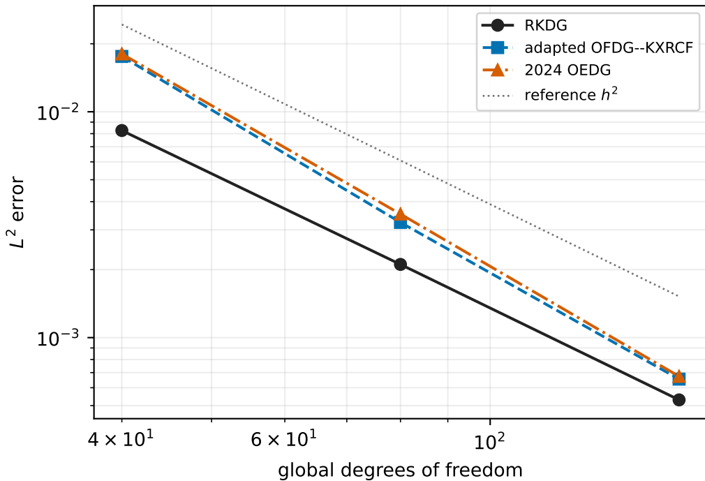
advection 1d, p^1
