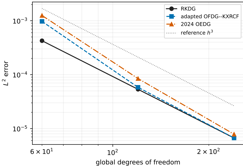
advection 1d, p^2
