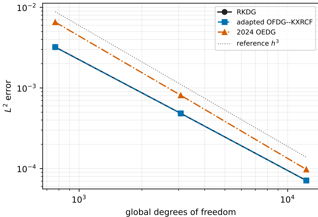
advection 2d triangular, P^2
