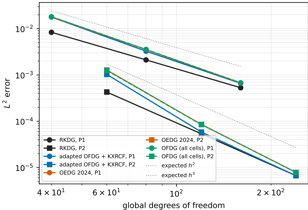
advection superconvergence
