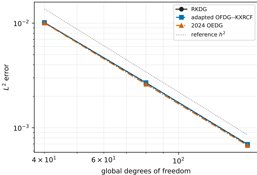
burgers smooth, P^1
