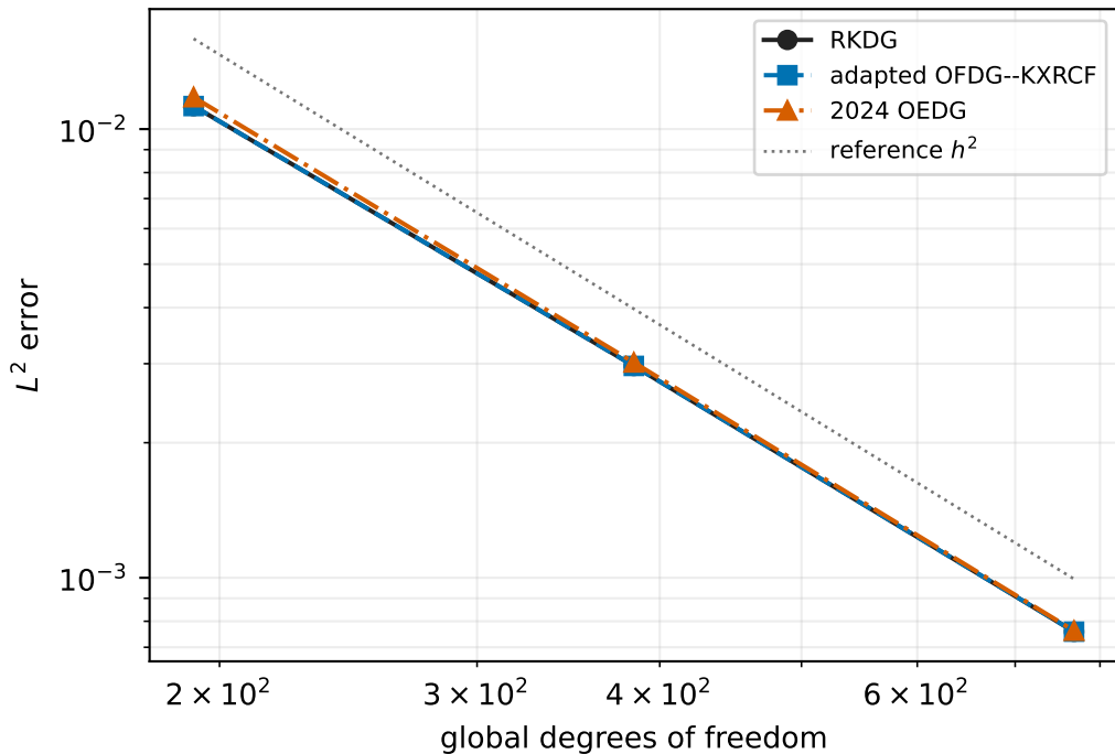
euler smooth 1d, p^1
