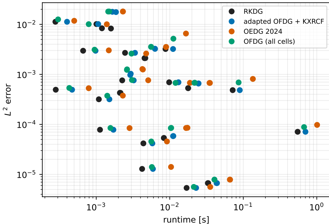
Accuracy-cost comparison
