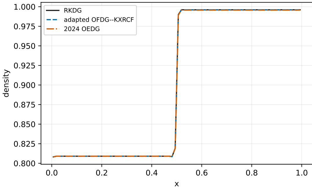
2D Riemann horizontal cut, P^1
