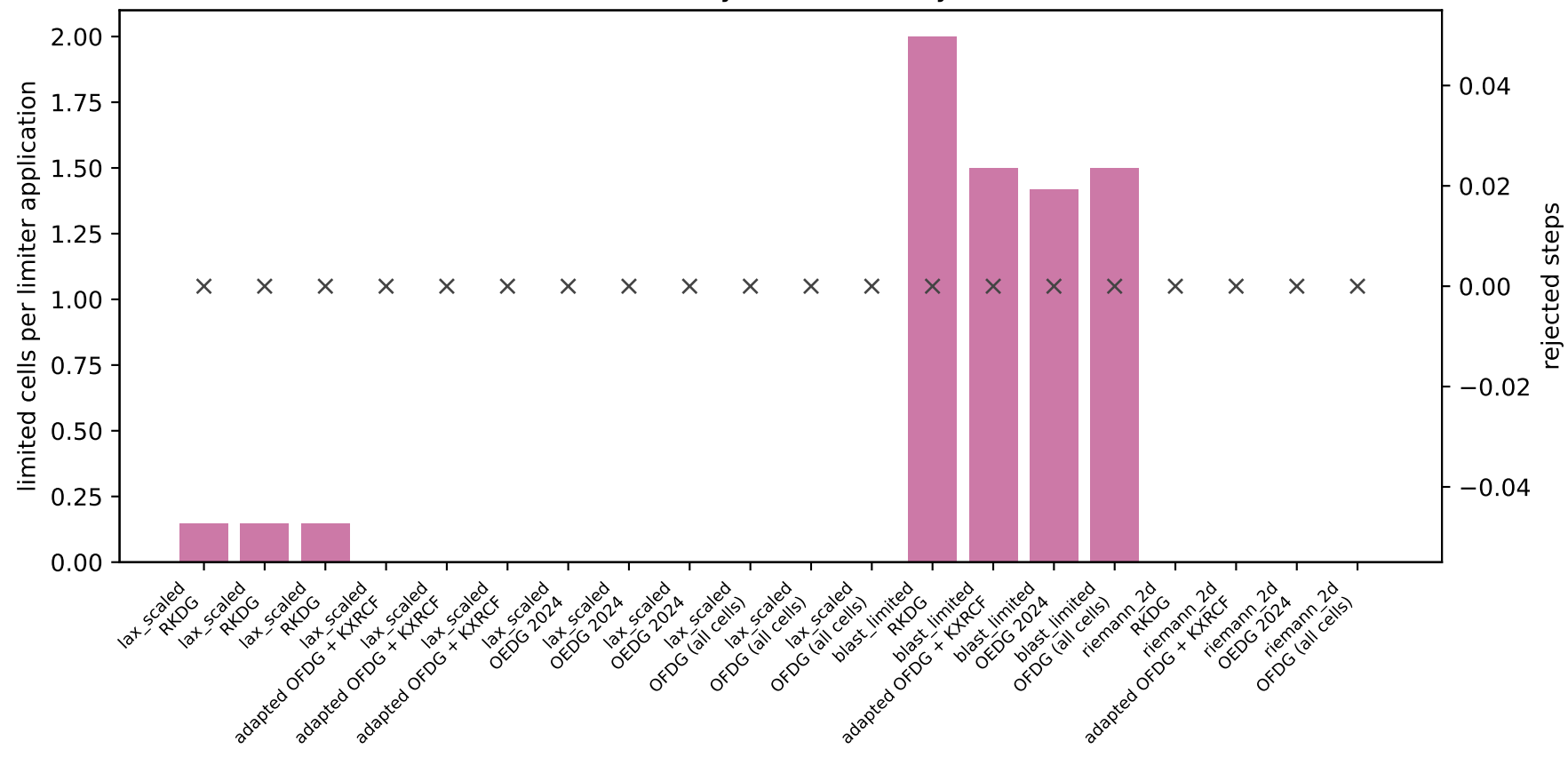
Positivity-limiter activity
