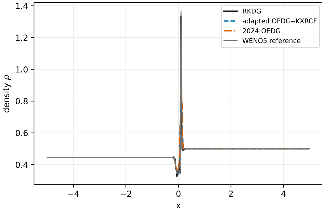
Scaled Lax problem, \lambda = 1, P^2
