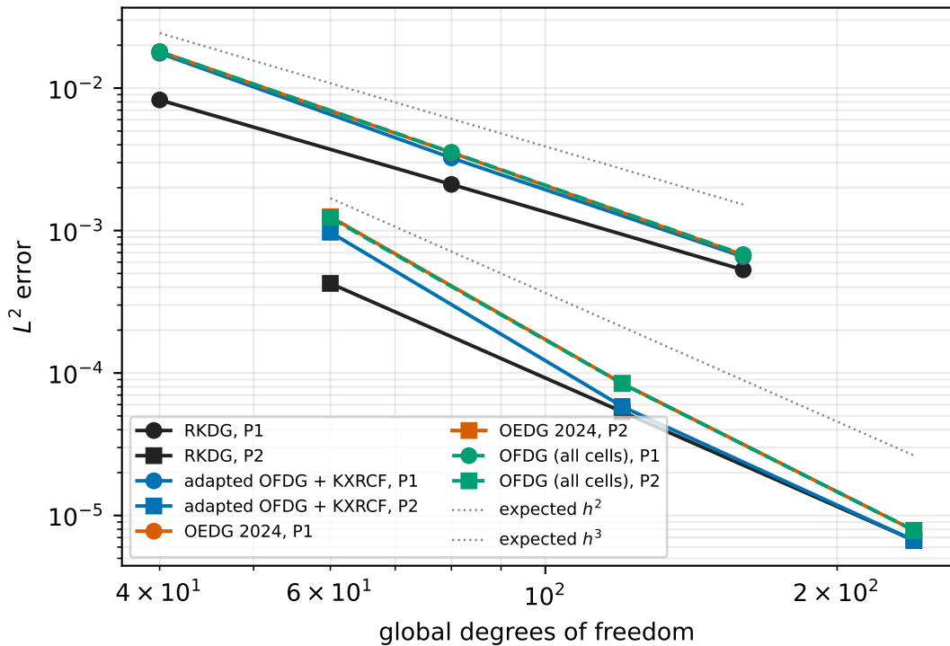
advection 1d
