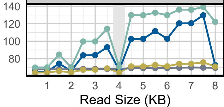
Latency
