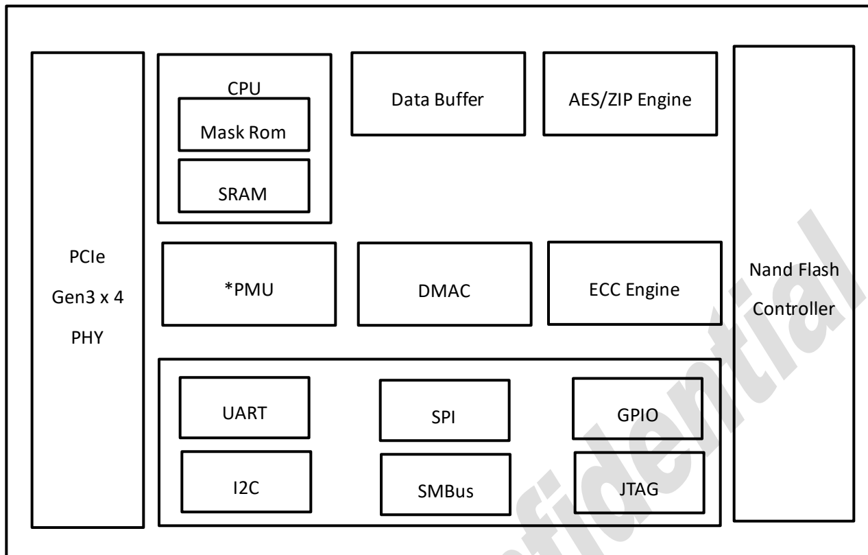
Figure 1-1 PS5015-E15T Controller Block Diagram
