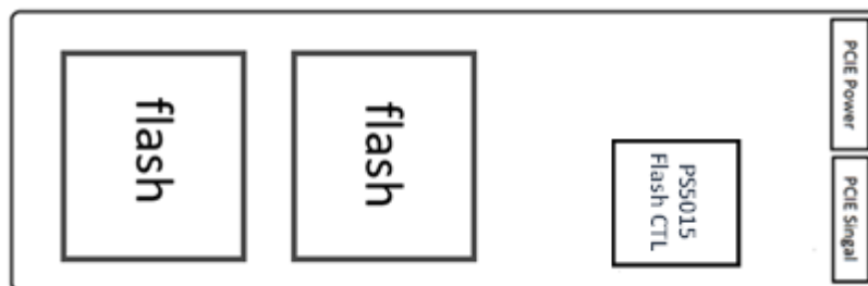
Figure 1-2 PS5015-E15T M.2 2280 Product Block Diagram
