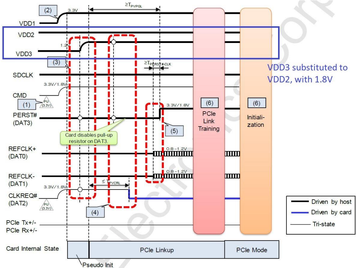
Figure 3-6 Direct PCIe Initialization
