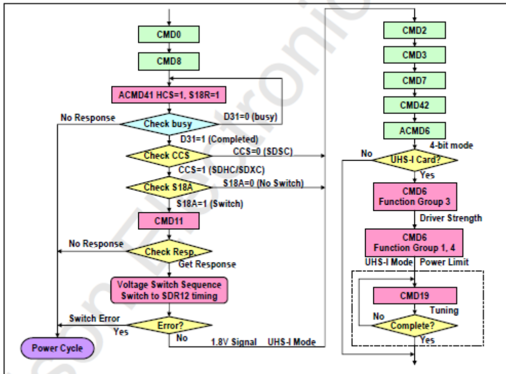
Figure 3-7 UHS-I Host Initialization Flow Chart
