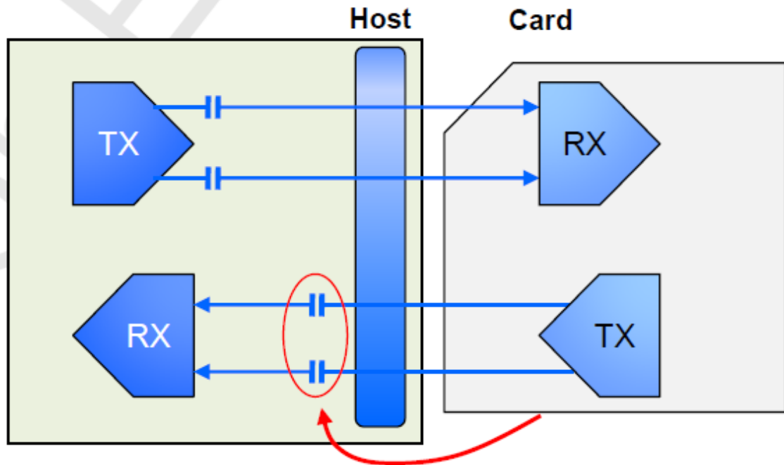
Figure 7-9 Placement of AC coupling capacitors of SD Express host
