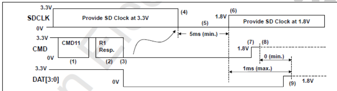
Figure 3-9 Signal Voltage Switch Sequence
