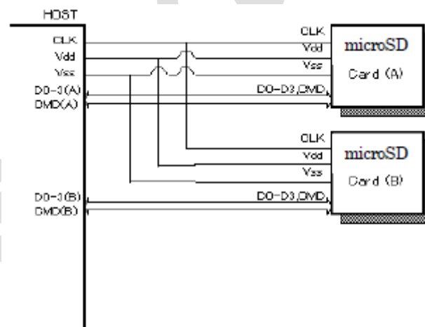
Figure 3-2 SD Memory Card System Bus Topology
