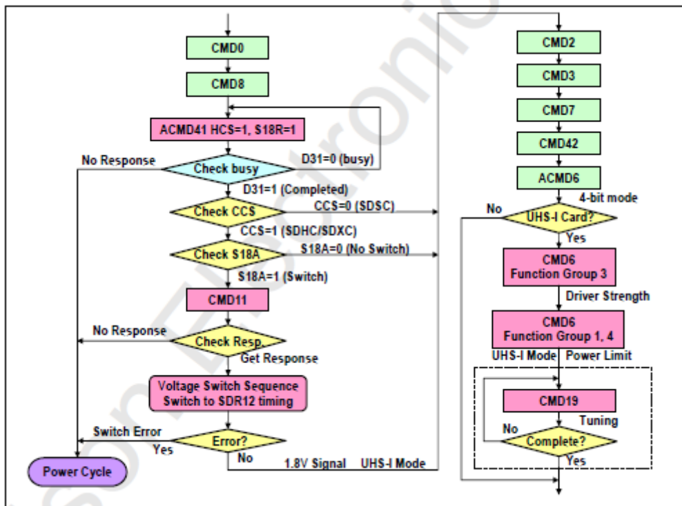
Figure 3-4 UHS-I Host Initialization Flow Chart
