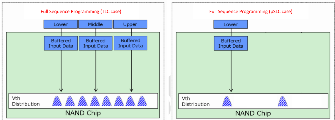
Figure 1-1 Cell Content of TLC (Left) and Pseudo SLC (Right)
