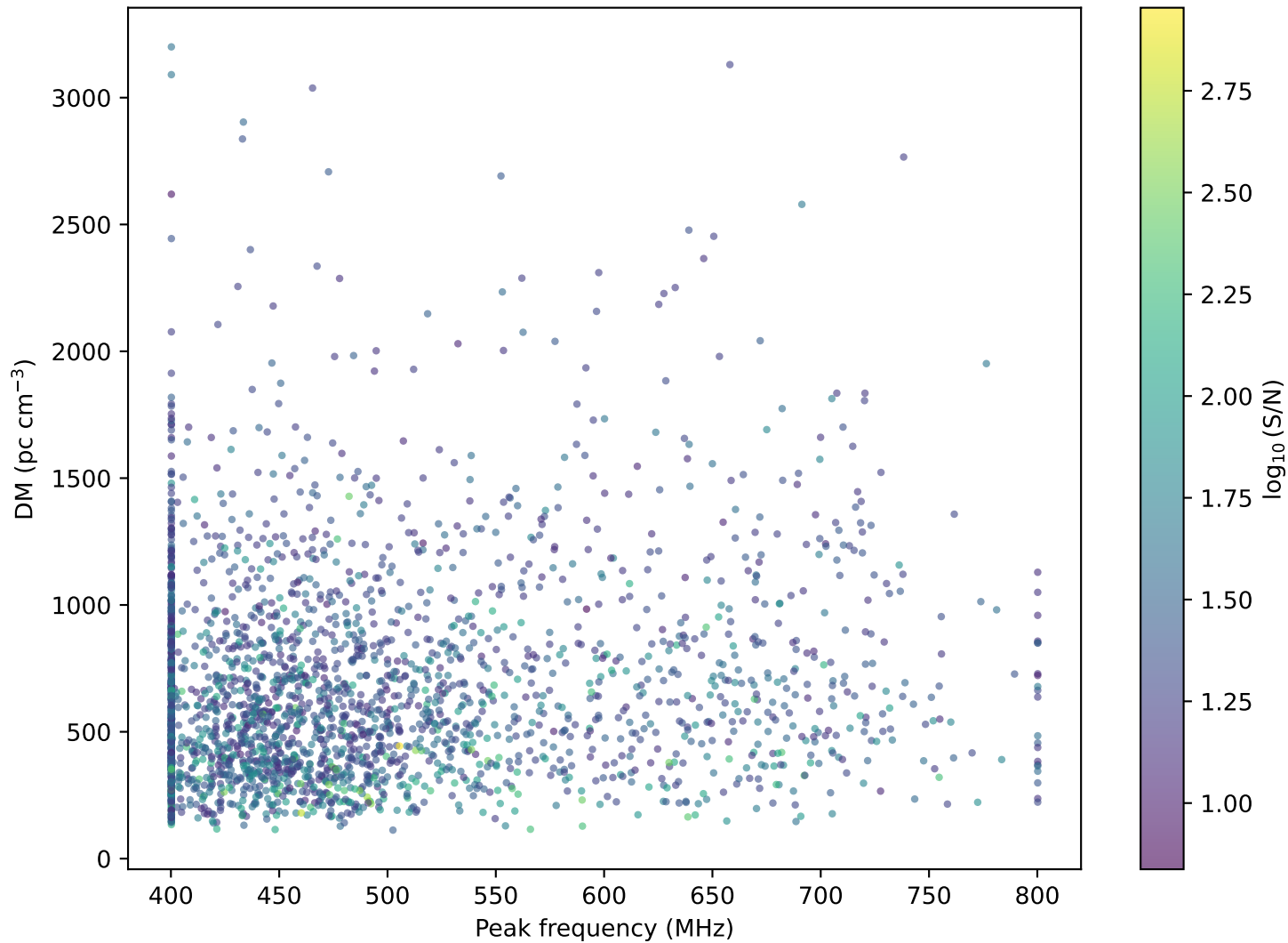
CHIME/FRB Catalog 2 — Peak frequency vs DM
