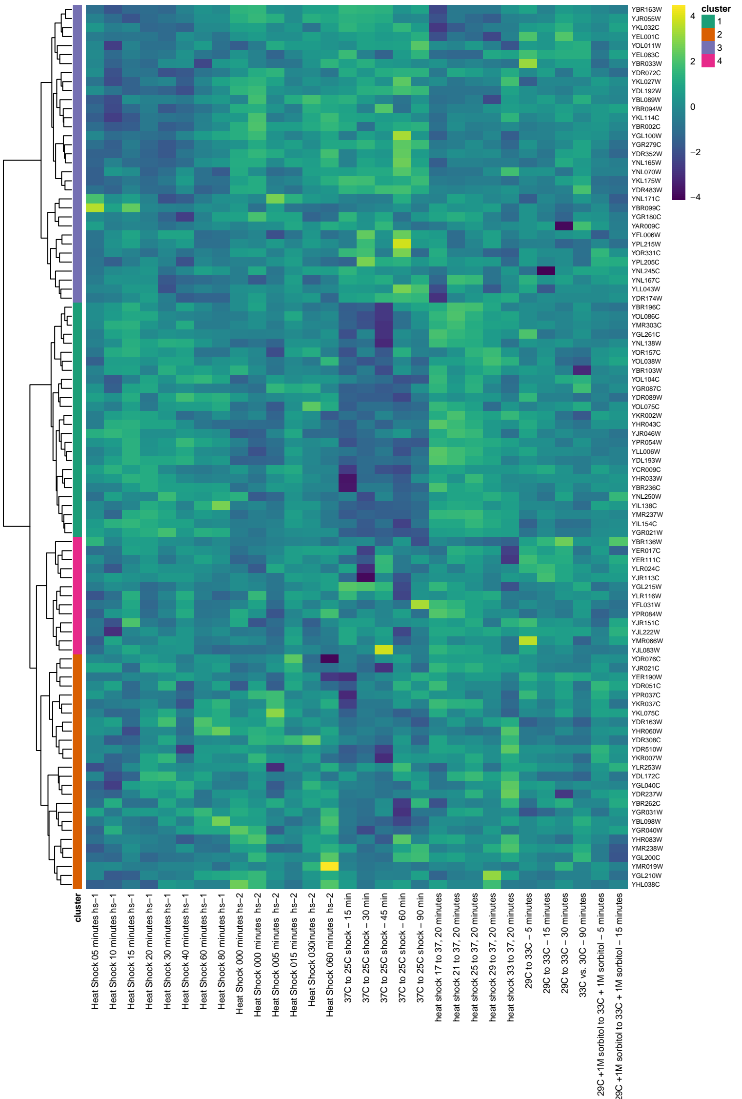
Yeast stress response, CV top200 (Gasch et al. 2000)
