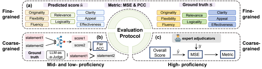
Figure 2: The three-modular evaluation protocol to assess the performance of scoring model. This evaluation protocol validates system robustness across varying annotation granularities (Fine vs. Coarse) and proficiency levels (High vs. Mid-Low). (a) Fine-grained evaluation measures the alignment of eight-dimensional predictions with human expert annotations using Mean Squared Error (MSE) and Pearson Correlation Coefficient (PCC). (b) Coarse-grained evaluation in the mid-to-low proficiency range. Given the instability of absolute scoring for lower-quality responses, we utilize Pairwise Accuracy (ACC) to assess the model’s capability to correctly rank synthetic sample pairs. (c) Coarse-grained evaluation in the high-proficiency range. We benchmark the model’s predictions against authentic top-tier expert adjudicator scores using MSE.
