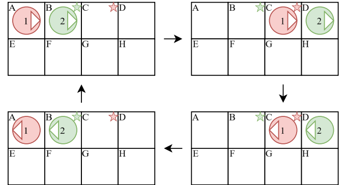
Figure 3. PIBT T cannot ensure that all agents reach their goals simultaneously
