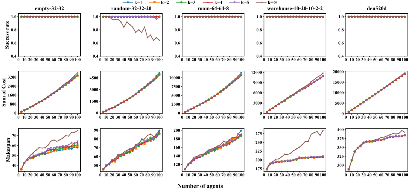
Fig. A1: Success rate, sum of costs and makespan of PIBT* with different k values.
