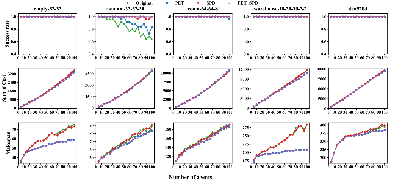
Fig. A2: Ablation experiment of SPD and PET in 5 different maps.
