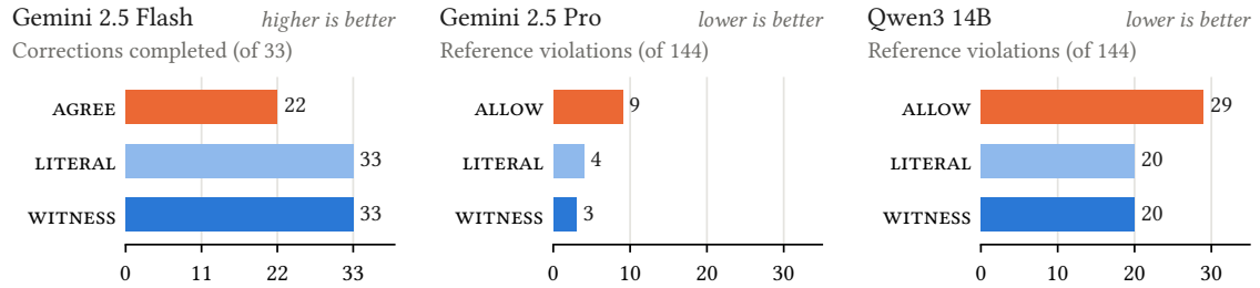
Same saved proposals within each panel. Baseline: AGREE for Flash, ALLOW for Pro and Qwen. Counts pool three repetitions of the 48 cases.
