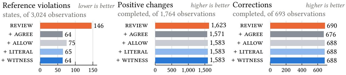
Fig. I1. Admission applied to saved REVIEW proposals: the AGREE and ALLOW bounds and the two evidence checks. The reference-violation endpoint follows the fixed state reference, including exact tuple mismatches. The same 21 configurations and all three repetitions appear in every bar; denominators are 3,024 for reference violations, 1,764 for positive changes, and 693 for corrections. Table I8 and Figure I2 report every configuration.
