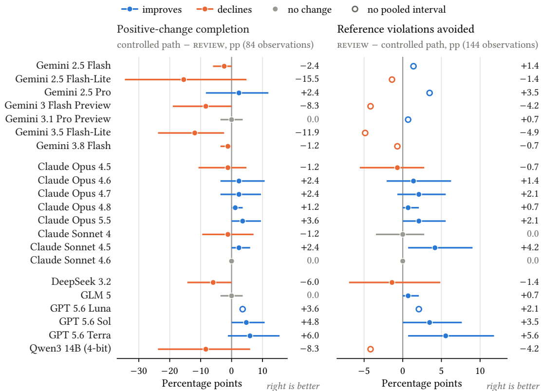
Fig. G1. Effects of the complete pipelines on the same 48 cases over three repetitions, oriented so that improvement is to the right (more positive completions and fewer reference-violating states). Positive completion uses 84 observations from 28 cases, and the reference-violation endpoint uses 144 observations from 48 cases. Blue marks improvement, orange decline, and gray no change; values at the right are point estimates in percentage points. Lines show the matching archived pointwise 95% case-cluster intervals, and open points mark configurations without a complete pooled interval.
