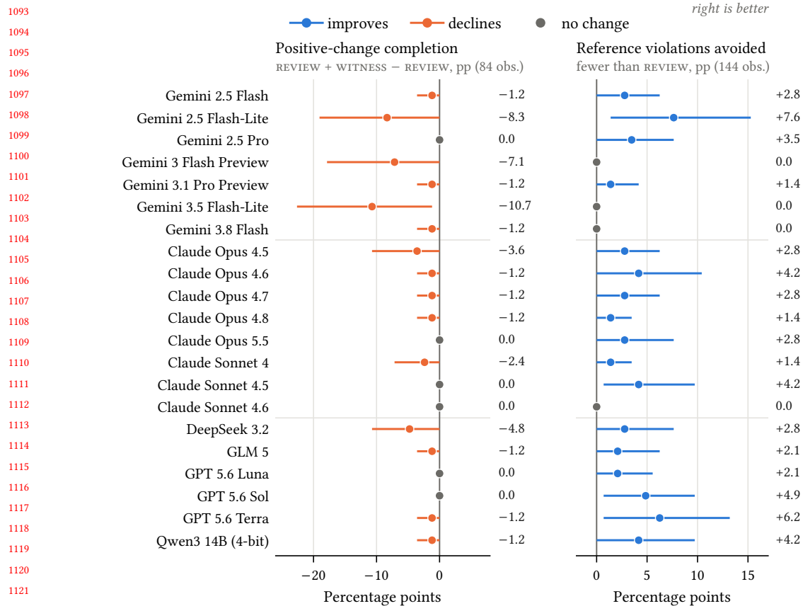
Fig. 12. REVIEW + WITNESS minus REVIEW, oriented so that improvement is to the right. Blue marks improvement, orange decline and gray no change; values at the right are point estimates in percentage points. Intervals cluster the three repetitions within each original case and are exploratory pointwise intervals. Both favorable restraint and unfavorable completion effects are shown.
