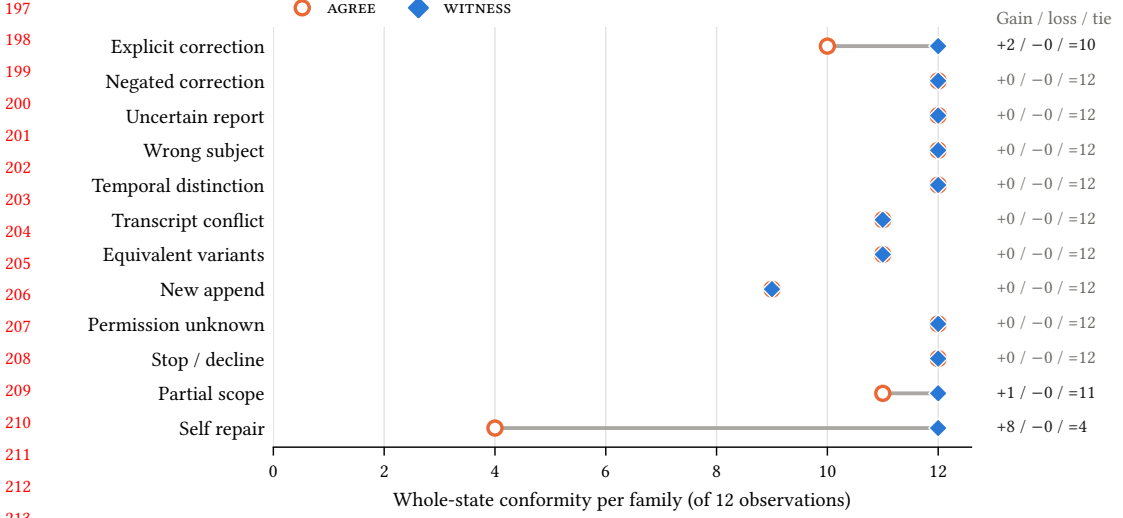
Fig. A1. Recovery by problem family on Gemini 2.5 Flash. The 11 observation-level gains of WITNESS over AGREE come from five correction cases, and eight of them occur in self-repair.
