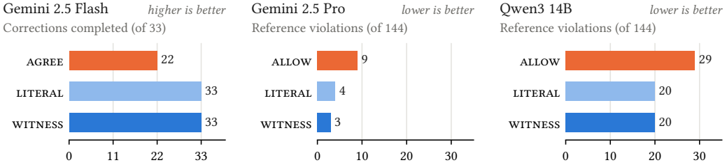
Same saved proposals within each panel. Baseline: AGREE for Flash, ALLOW for Pro and Qwen. Counts pool three repetitions of the 48 cases.
