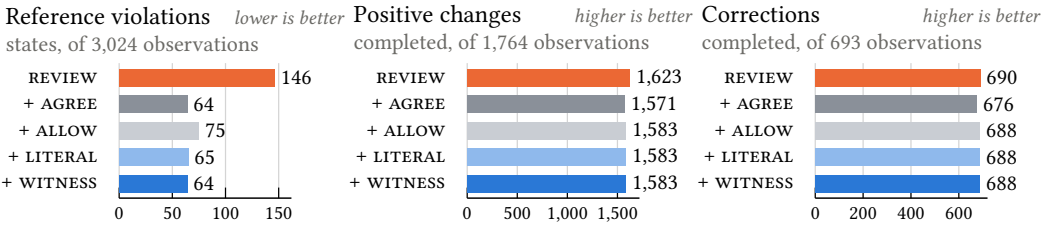
21 configurations × 48 cases × 3 repetitions. Invalid final outputs: 21 under REVIEW, 29 under each admission rule.
