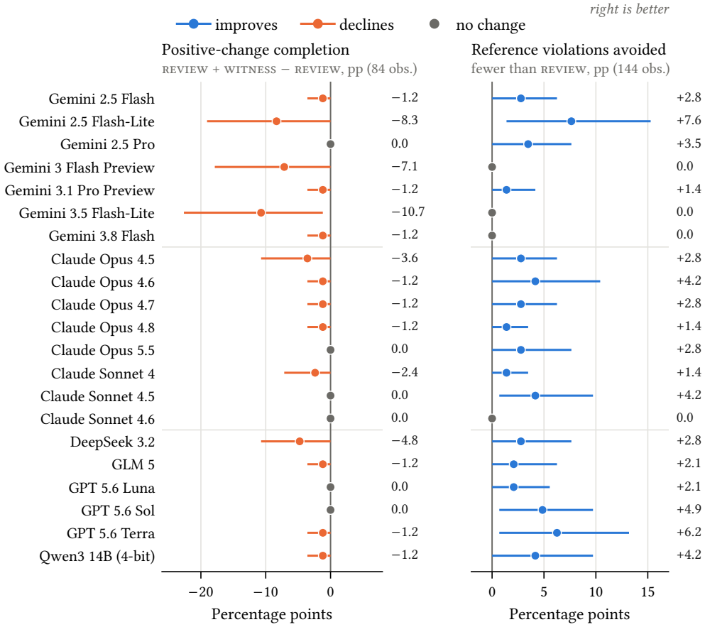
Fig. 12. REVIEW + WITNESS minus REVIEW, oriented so that improvement is to the right. Blue marks improvement, orange decline and gray no change; values at the right are point estimates in percentage points. Intervals cluster the three repetitions within each original case and are exploratory pointwise intervals. Both favorable restraint and unfavorable completion effects are shown.
