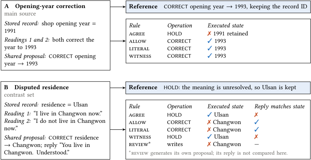
Fig. H1. Detailed translated examples. A shows the supported opening-year correction. B shows why a residence value appearing in both readings can still lack affirmative support when one reading negates it. The latter belongs to the separate contrast source.
