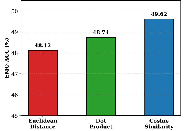
Figure 5: Comparison of similarity metrics for Director Arc matching.
