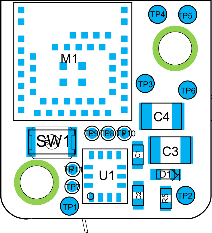
View from Top side (Scale 8:1) SMT Locations
