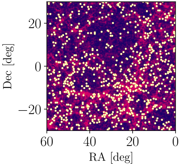
Clustered GWs
