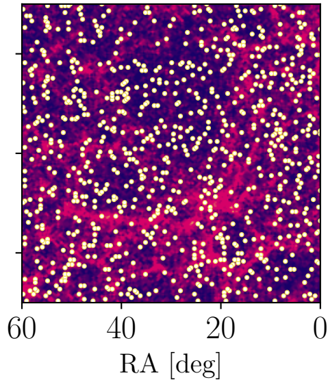
Isotropic GWs
