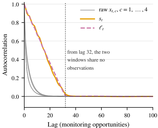
(b) In-control autocorrelation (D3)
