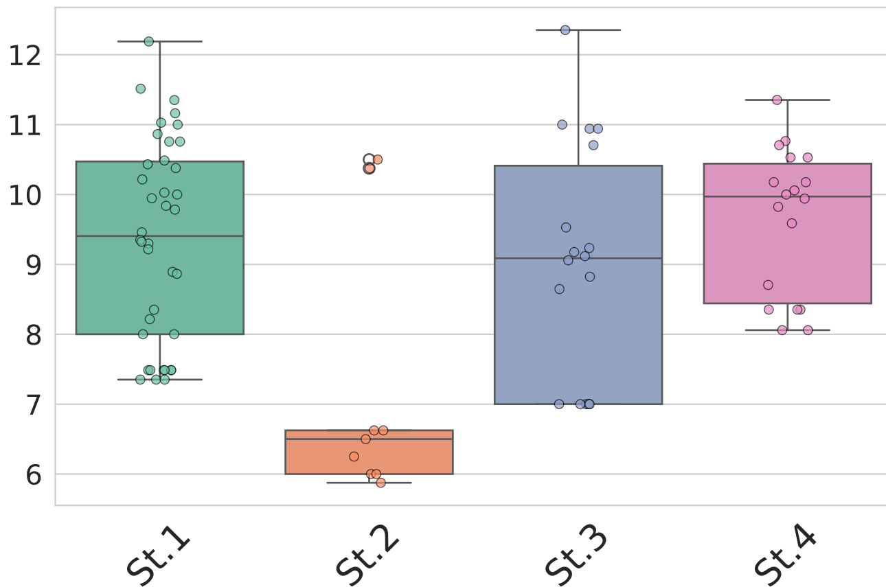
SHD
