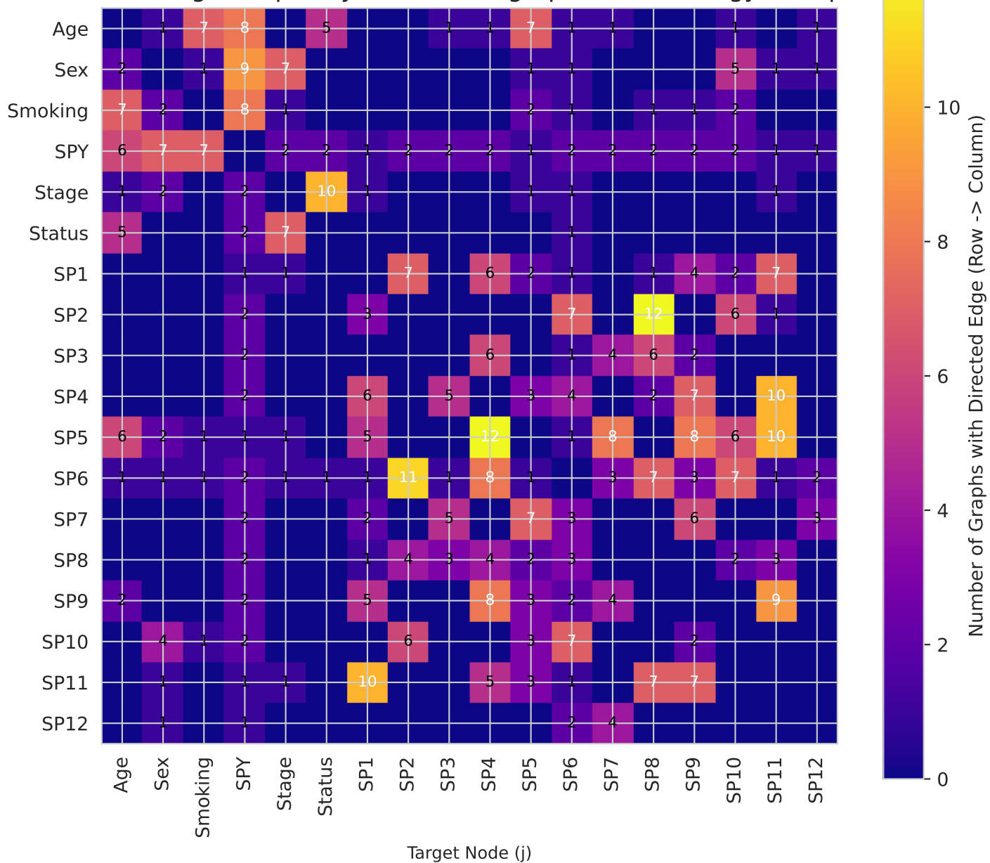
Directed Edge Frequency, Number of graphs: 18, Strategy: Complete
