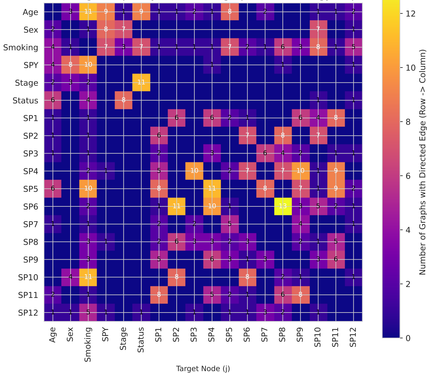
Directed Edge Frequency, Number of graphs: 18, Strategy: Imputed
