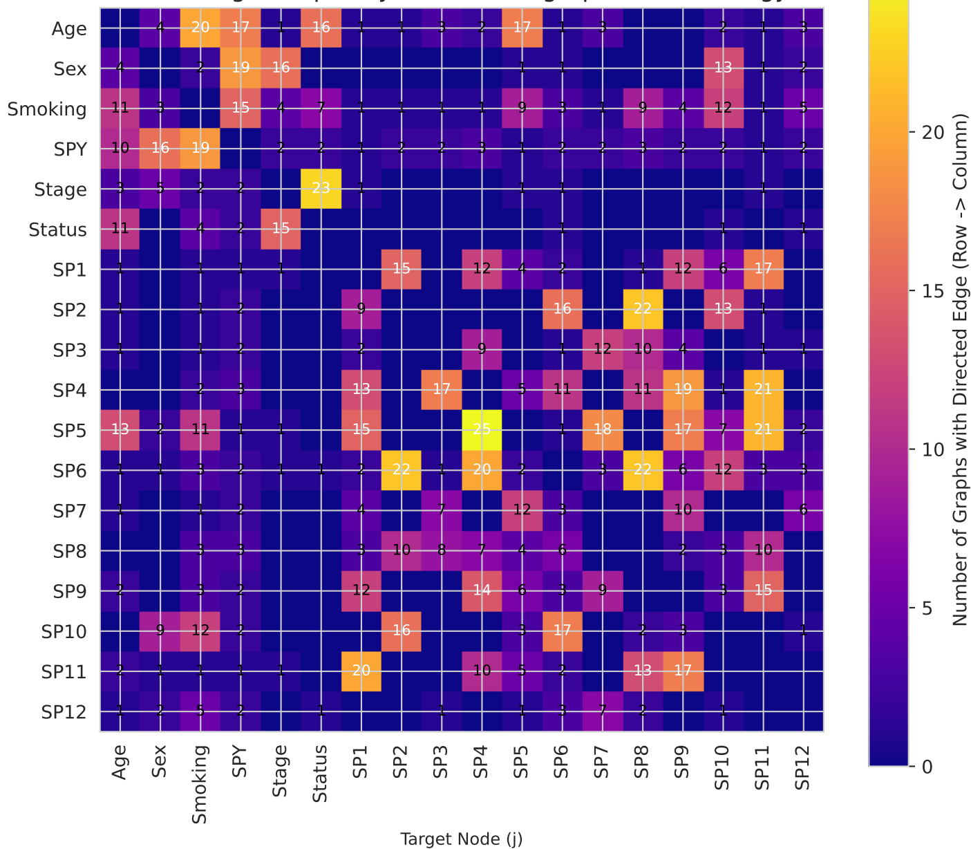
Directed Edge Frequency, Number of graphs: 38, Strategy: All
