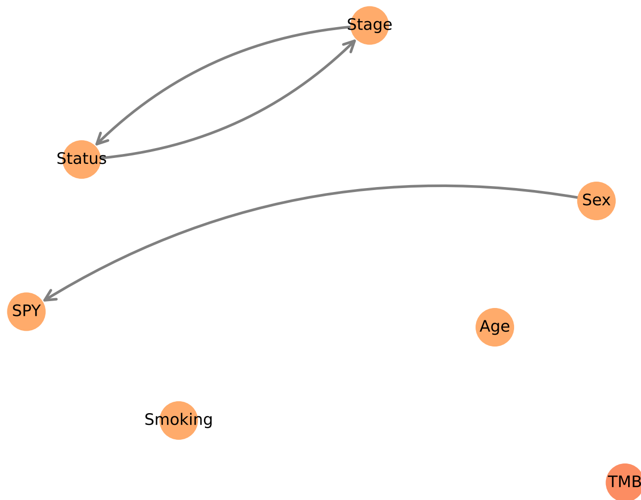
Directed edges (50% consensus)
