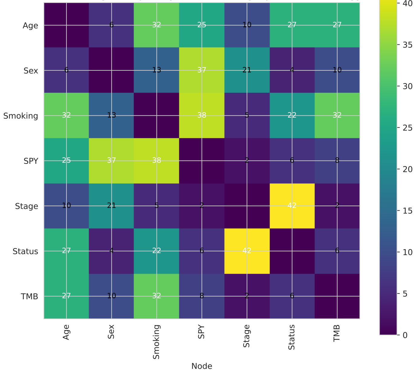
Undirected Edge Frequency, Number of graphs: 38, Strategy: All
