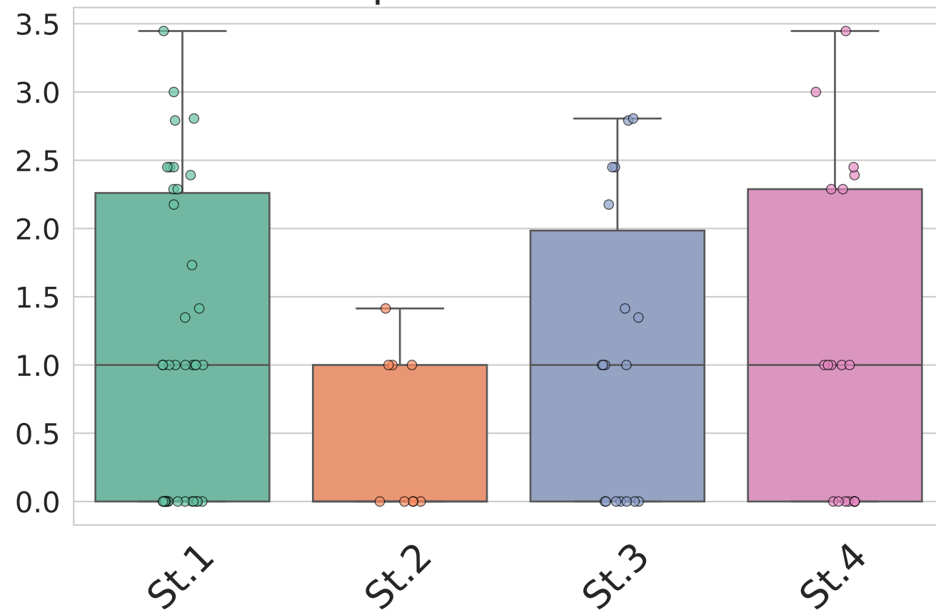
Spectral Radius
