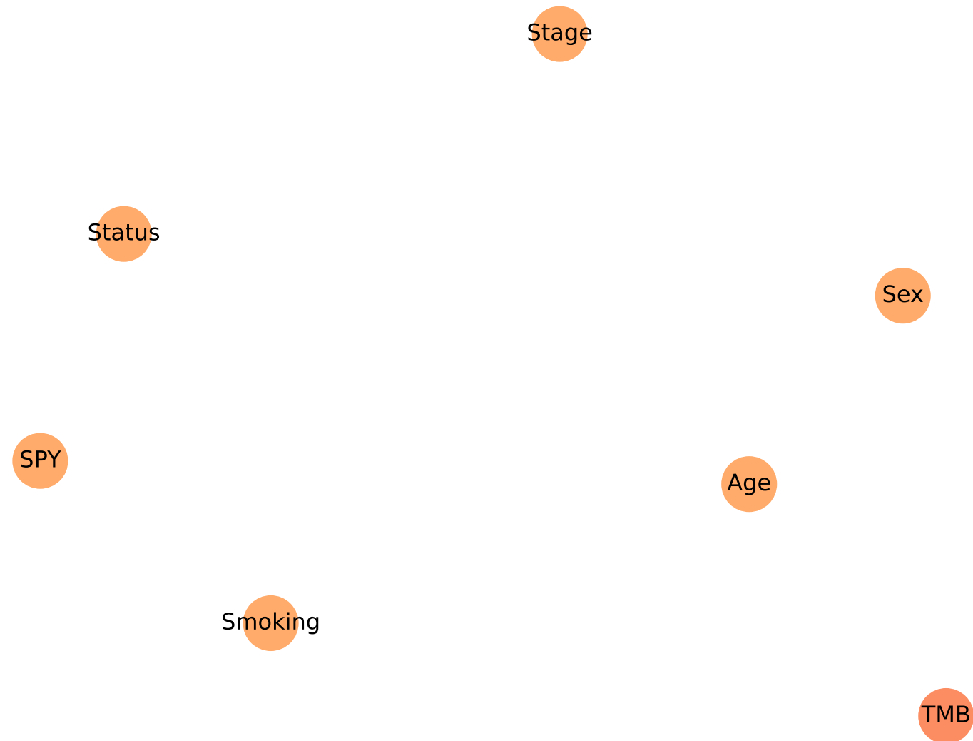
Directed edges (70% consensus)
