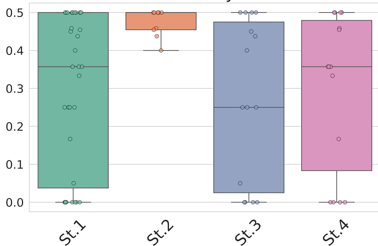
Directionality Index
