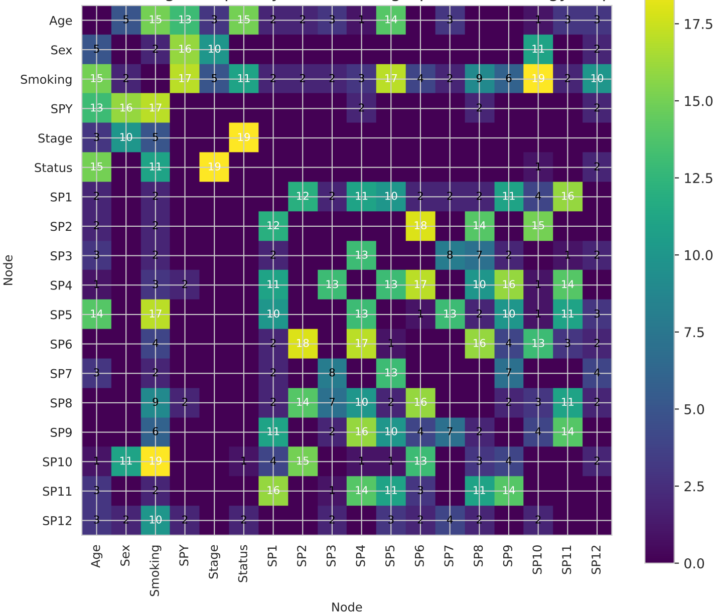
Undirected Edge Frequency, Number of graphs: 18, Strategy: Imputed
