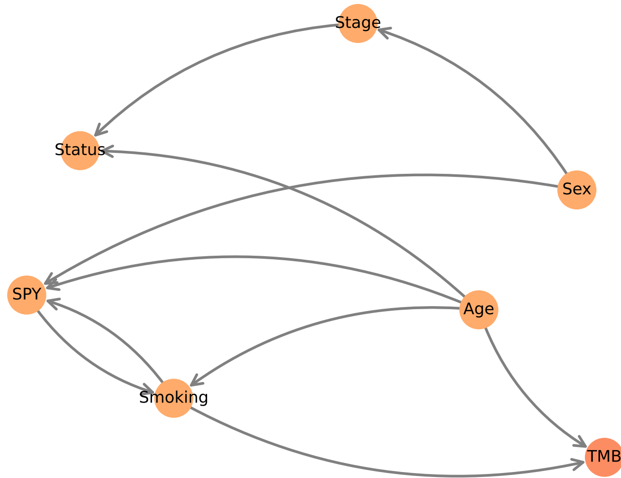
Directed edges (50% consensus)
