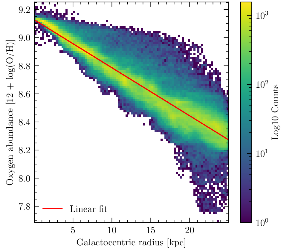
Oxygen abundance vs Galactocentric radius
