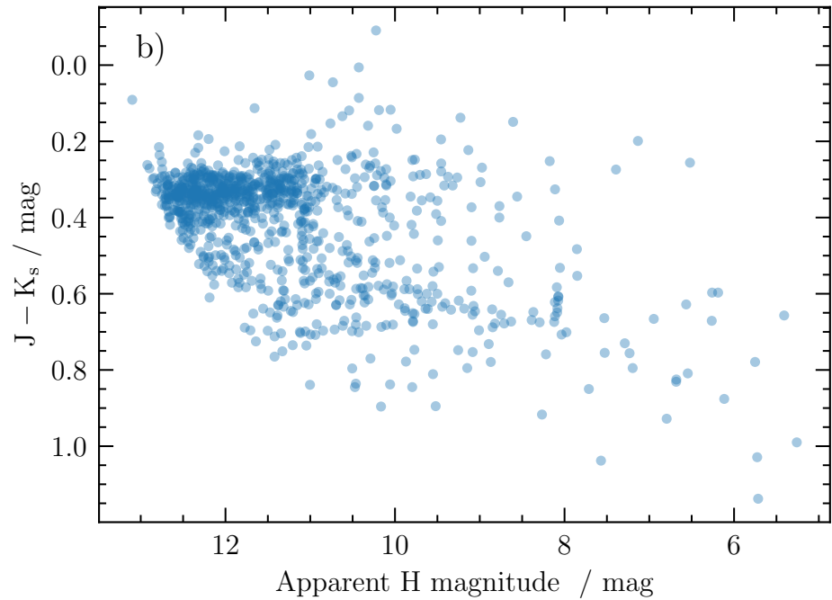
2MASS
