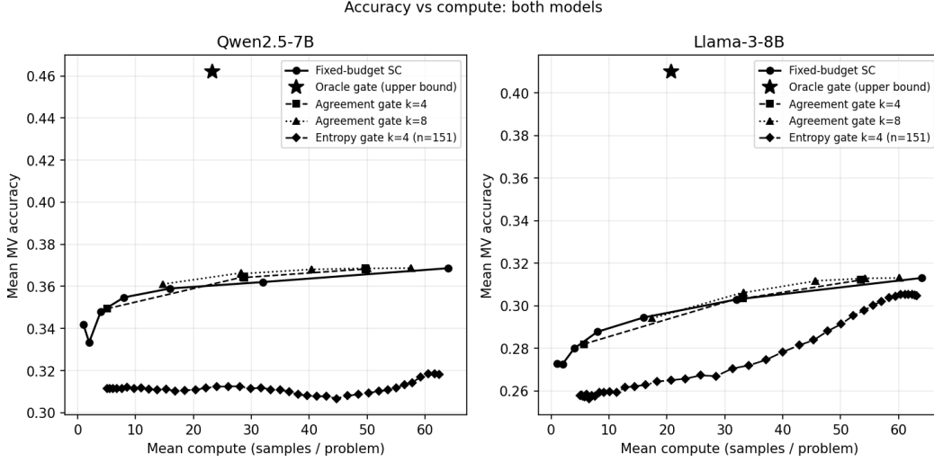
Figure 2: Accuracy vs mean compute: fixed-budget voting, the oracle upper bound, and the verifier-free agreement and entropy gates. The entropy series is computed on the confirmatory 151 only, a harder subset than the pooled 198 used for the other series, so its lower position does not by itself indicate a worse method.
