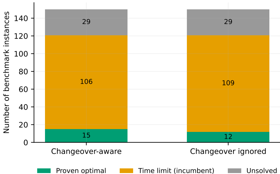
Solver outcomes under the time limit
