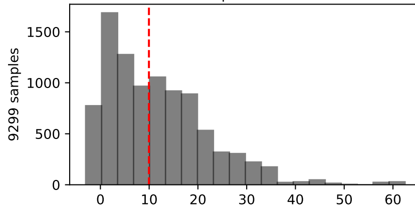
Median wind speed difference: 9.95
