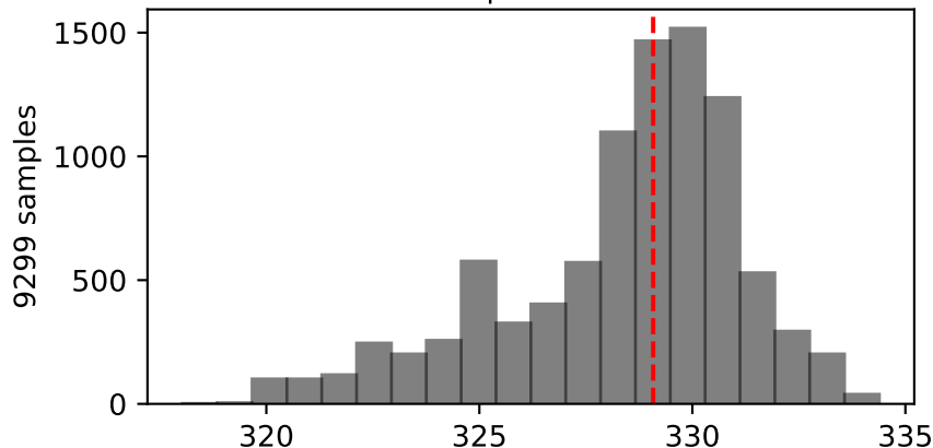
Median speed of sound difference: -17.14
