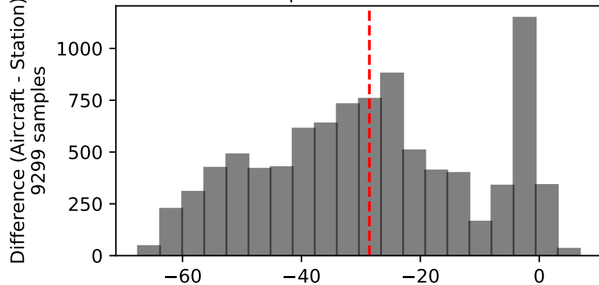
Median temperature difference: -28.57
