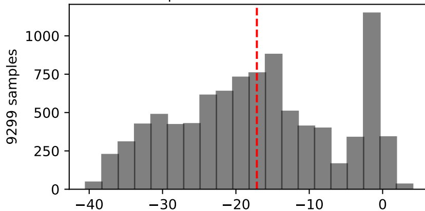
Median speed of sound difference: -17.14
