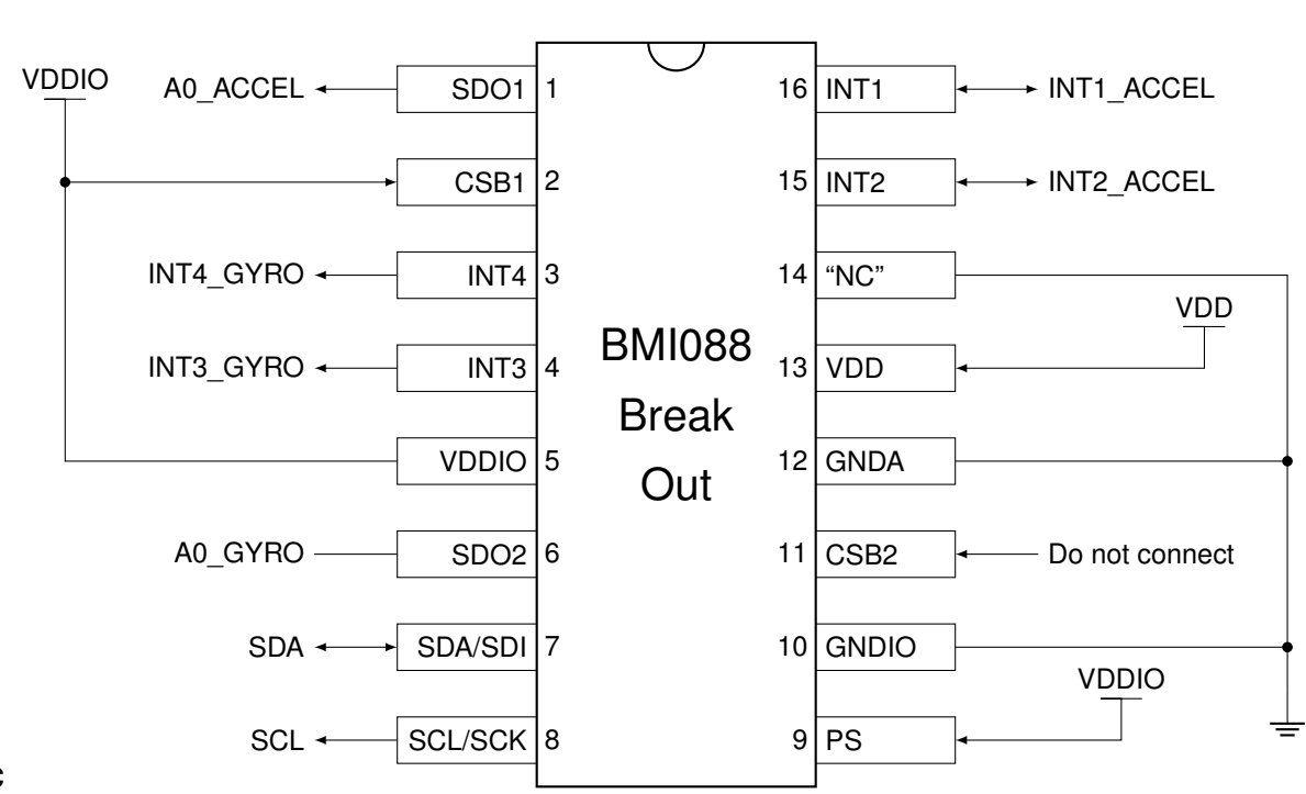
Connection diagram I 2 C
