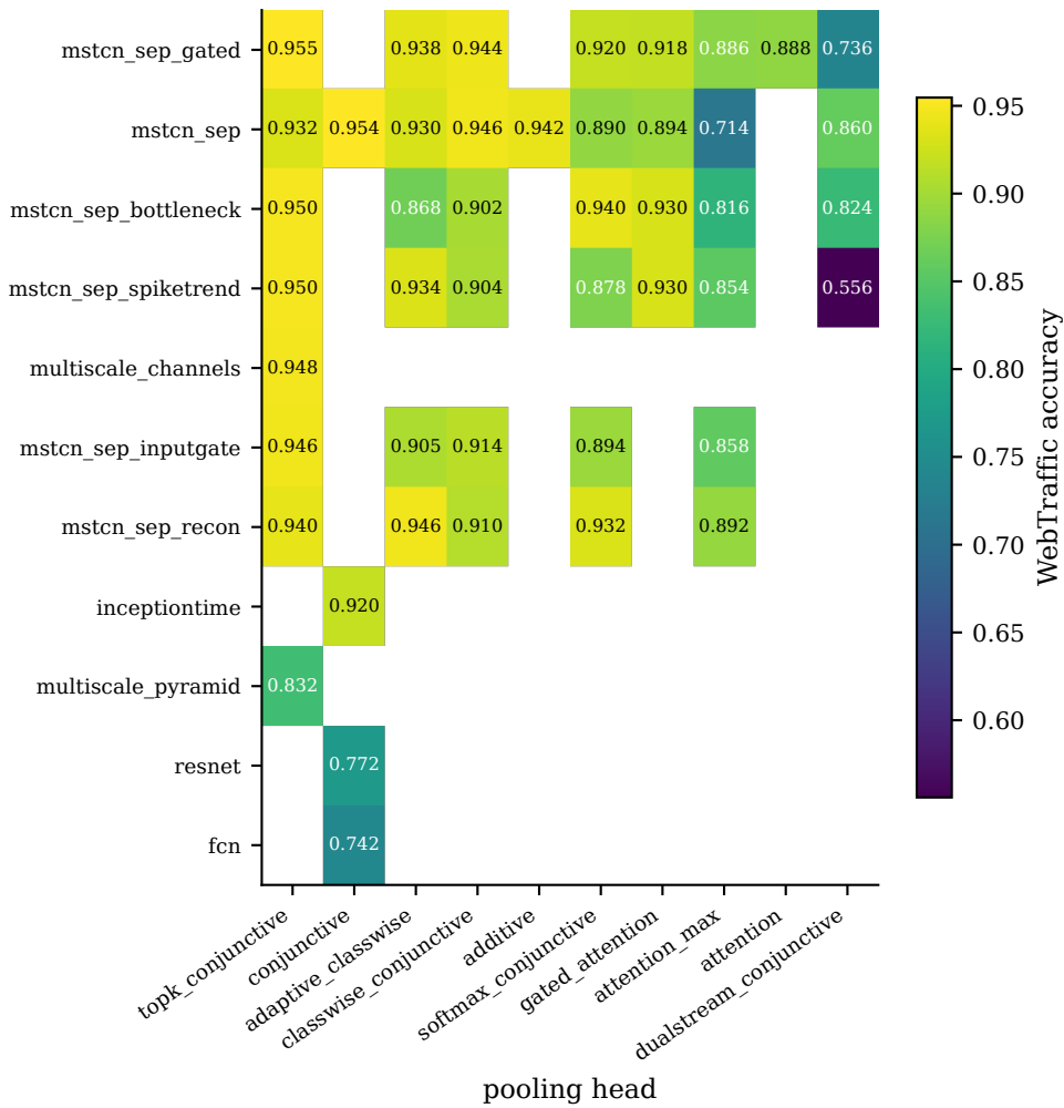
Best accuracy for each encoder x pooling combination
