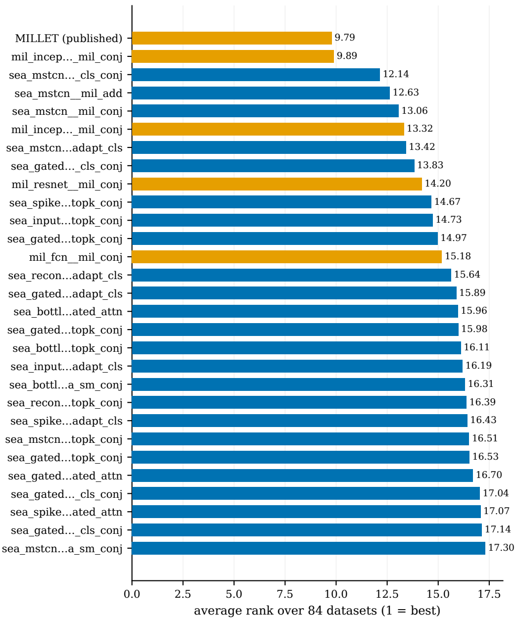
Average rank (accuracy)
