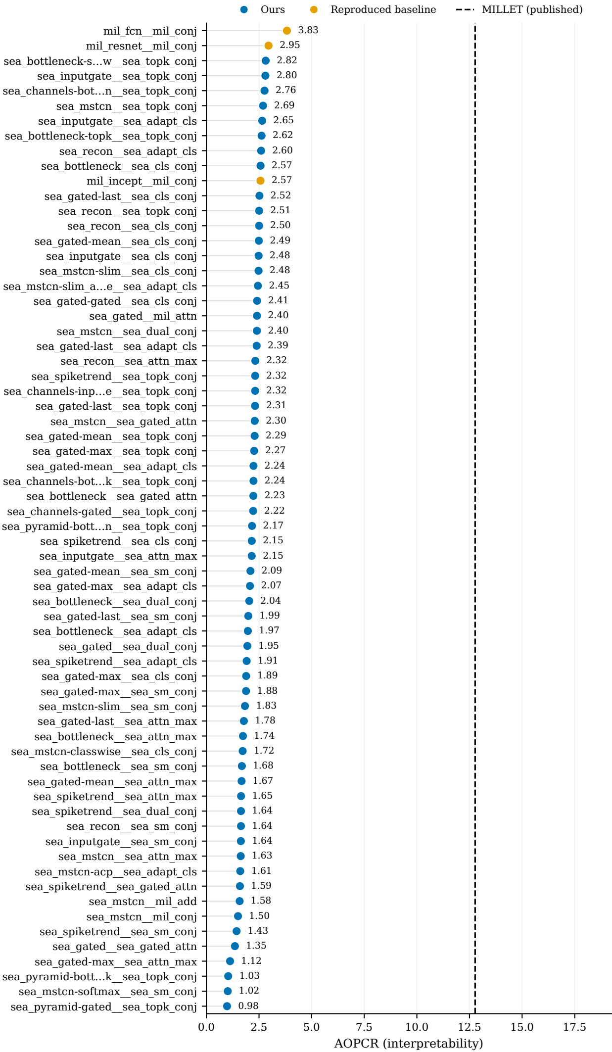
WebTraffic: AOPCR (all 66 models)
